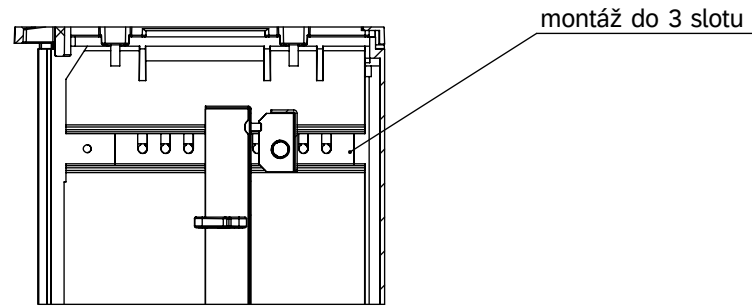
DETAIL C (1 : 5)
